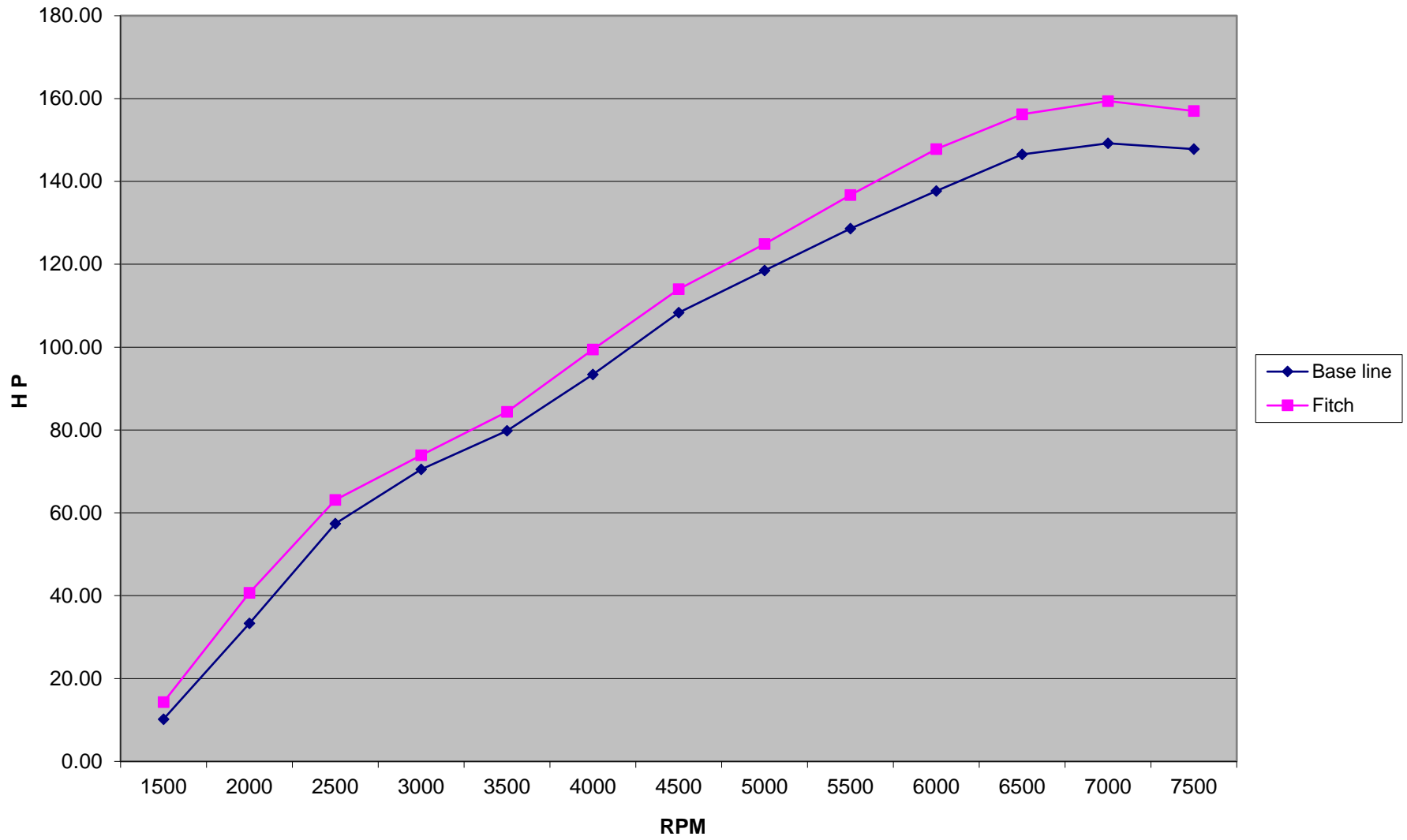
2008 Ford Focus HP Data Dastek Dynometer
